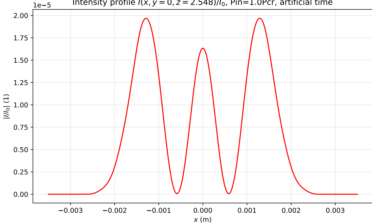
Intensity profile I(x, y = 0, z = 2.548)/I_0 , P_{in}=1.0P_{cr} , artificial time
